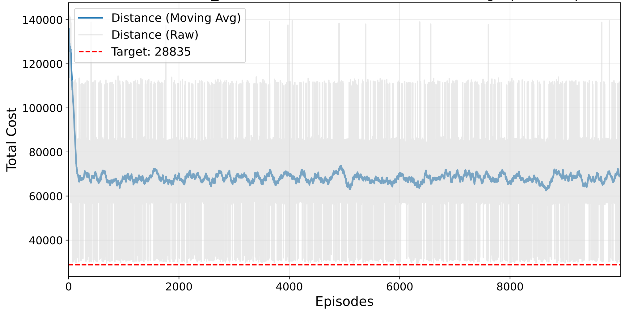
Final RANDOM_SEARCH Masked AutoRL-SOP Training - p43.3.sop
